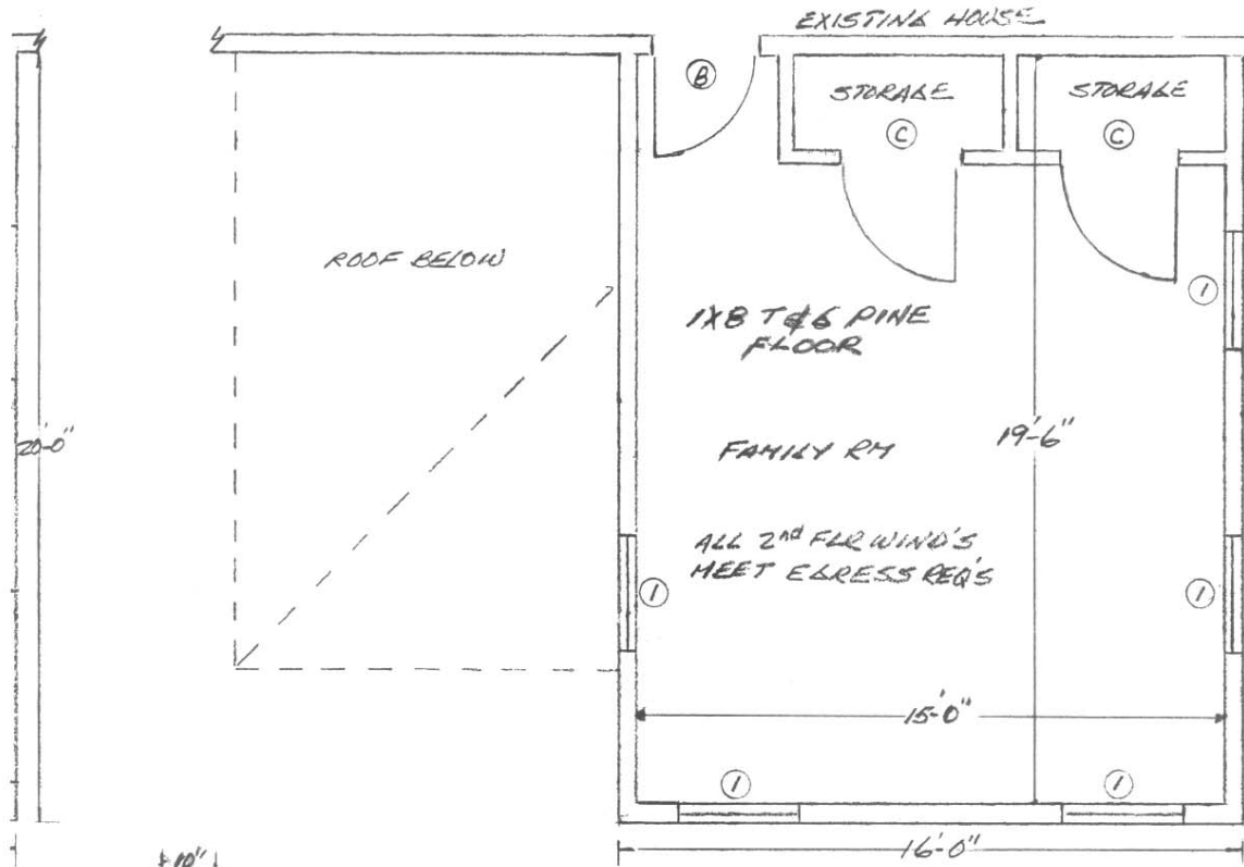
SECOND FLR PLAN SCALE: 1/4" = 1'-0"
