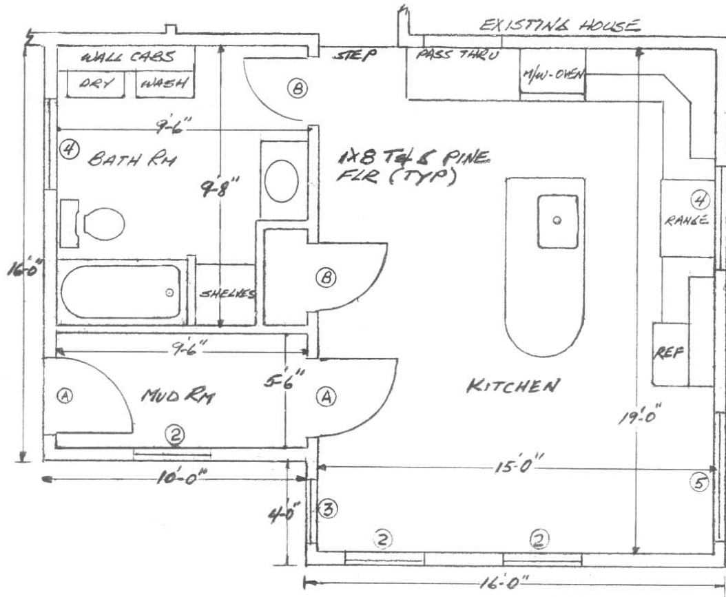
FIRST FLR PLAN SCALE: 1/4" = 1'-0"
